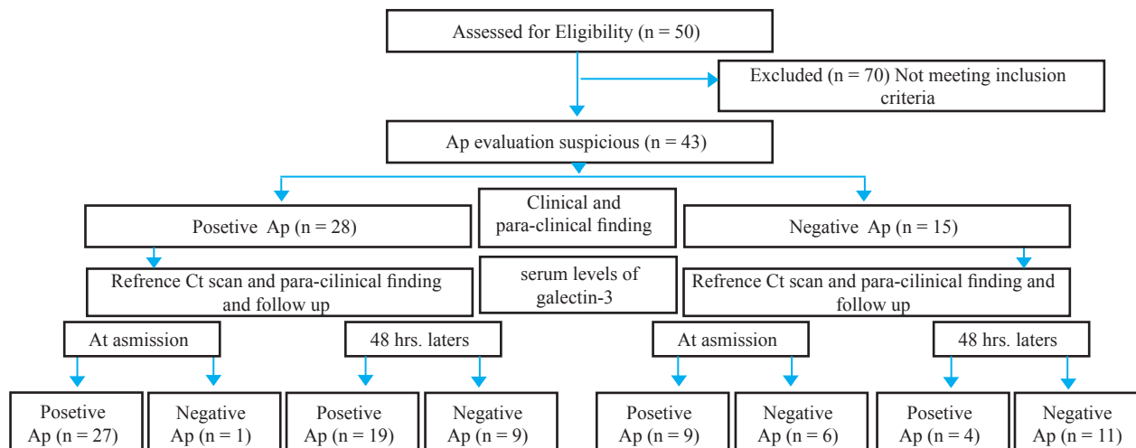
Fig. 1: Study flowchart
